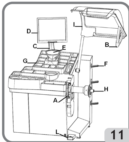
Main working elements of the machine (fig. 11)
